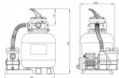
Sand filter dimensions
